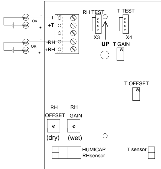
Figure 3.3 Electrical connections
